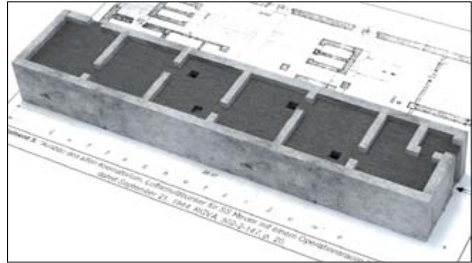
Figure 7: Air-raid shelter configuration
